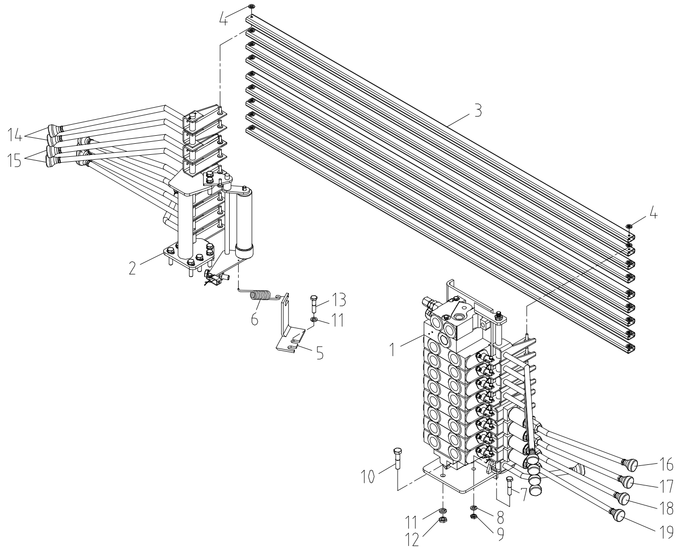
Fig. 3-4 SCS513 OPERATION MAIN ASS'Y
