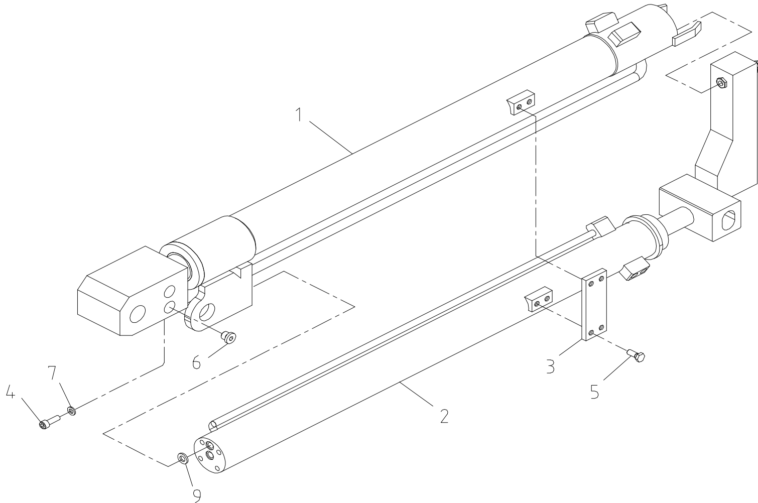
Fig. 1-1 SCS513 TELESCOPIC CYL' ASS'Y
