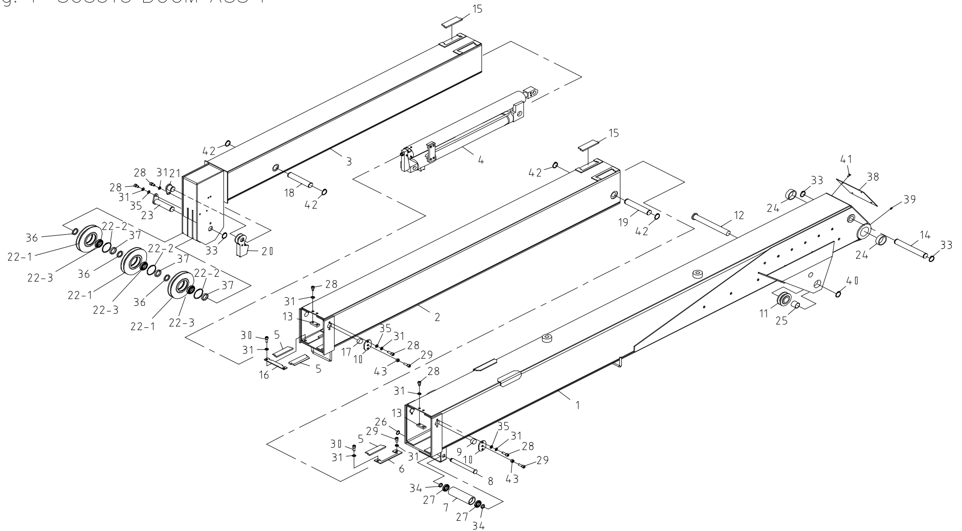
Fig. 1 SCS513 BOOM ASS'Y
